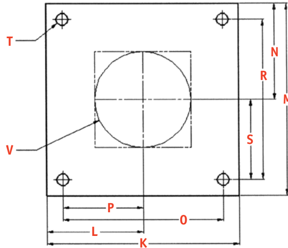
Top Flange Operator Side (Front)
