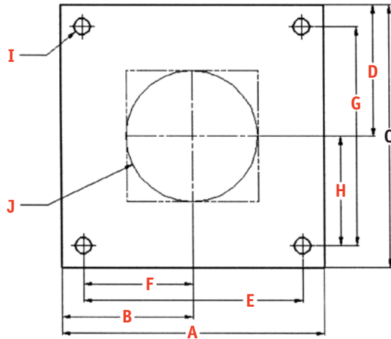
Bottom Flange Operator Side (Front)
